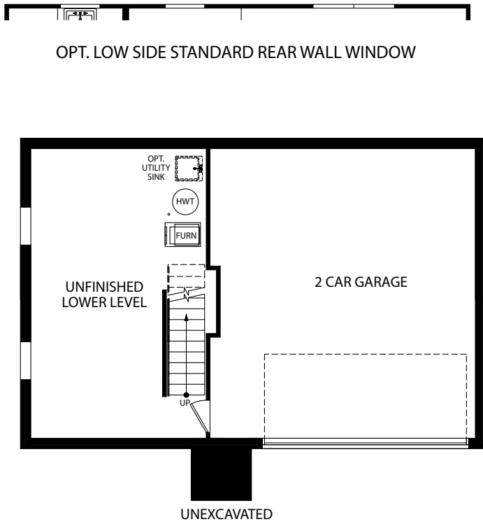
OPT. HIGH SIDE, FRONT ENTRY GARAGE
