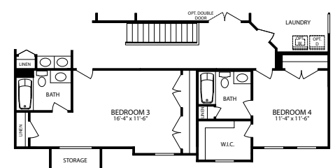
Opt. Princess Bath with Opt. Duke Bath
