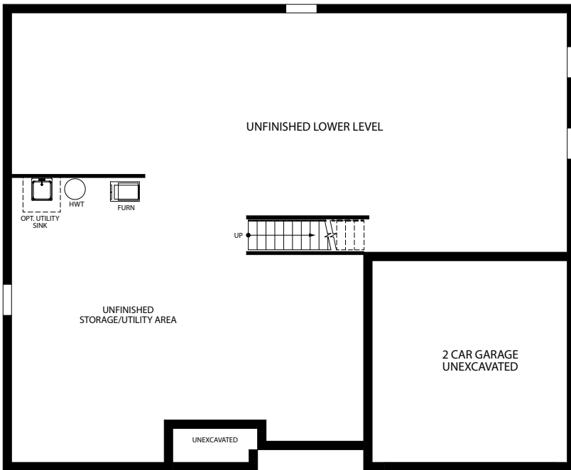
HIGH SIDE UNFINISHED LOWER LEVEL
