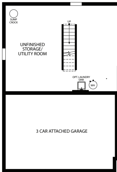
OPT. 3 CAR FRONT ENTRY GARAGE HIGH SIDE - UNFINISHED LOWER LEVEL
