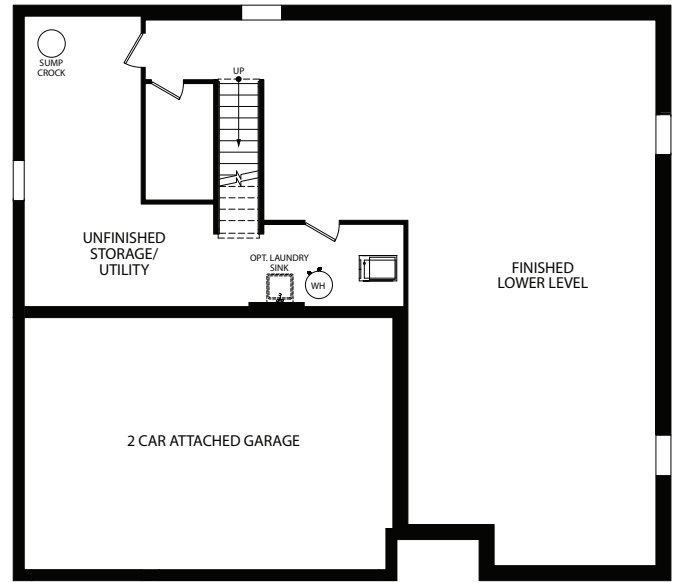
OPT. ELEVATION G FINISHED LOWER LEVEL HIGH-SIDE
